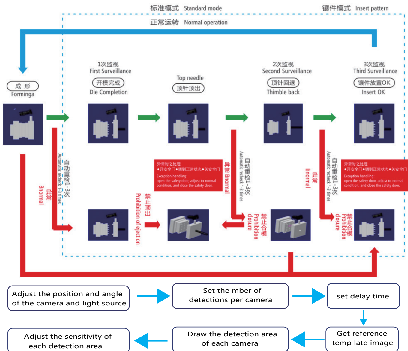
Monitor flowchart
